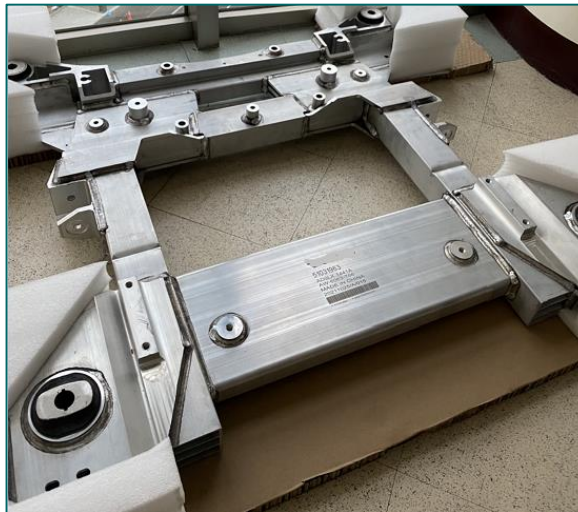
Subframe Welding Assembly
