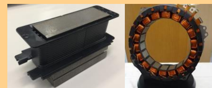
Electric Vehicle Motor Coil Parts (Nifco)
