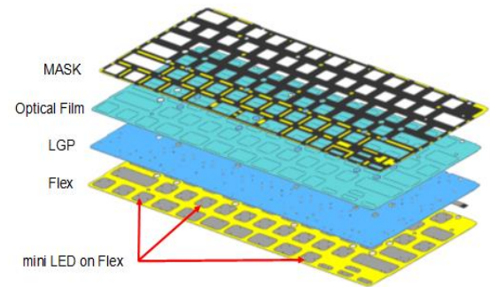
Explosion Drawing :
