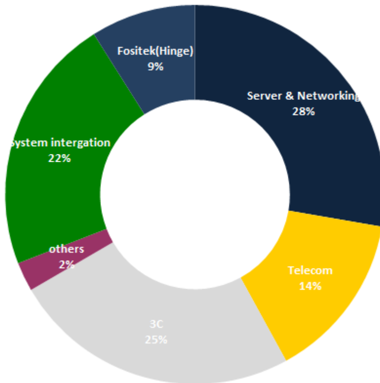
2022Y
