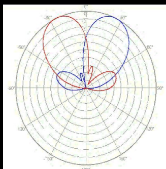
1L+2 Twin beam
