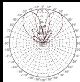
1L+2 Triple beam
