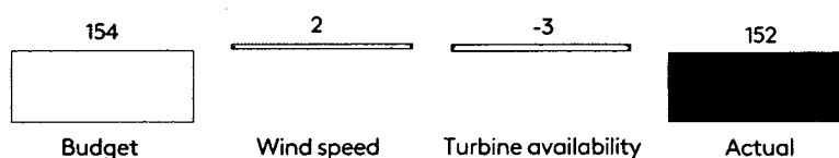
Figure 11: 2023 offshore wind output variance to budget
