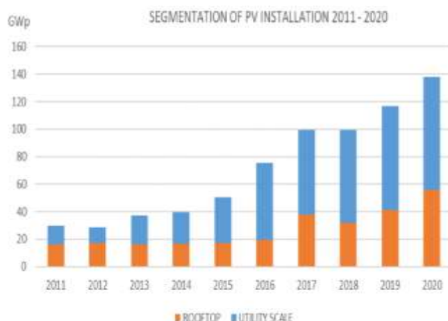
EVOLUTION OF ANNUAL PV INSTALLATIONS
