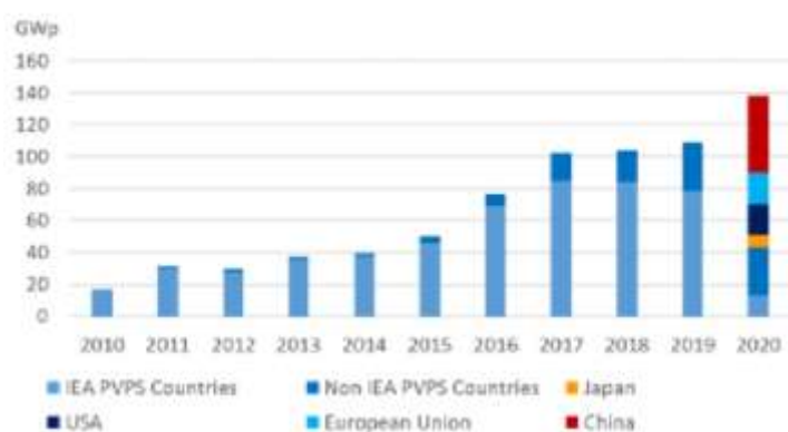
EVOLUTION OF ANNUAL PV INSTALLATIONS
