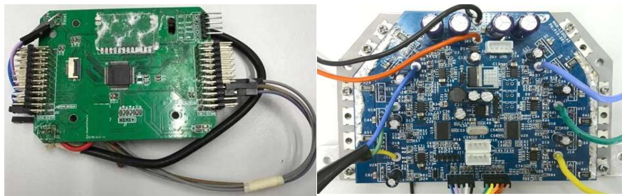
Wheeled Mobile Robot Solution
