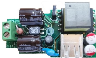
AD DC Medical Plug Wall 10W Adapter Solution
