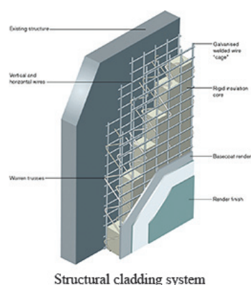
Structural cladding system
