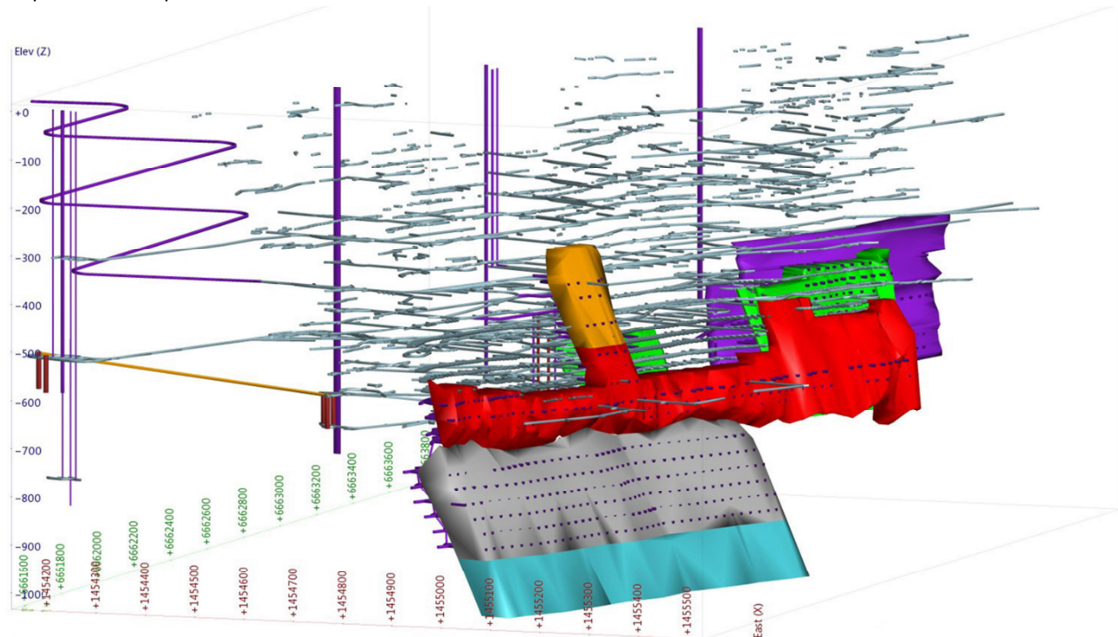
Three-Dimensional View of Grangesberg Showing Resource blocks, existing shafts and planned new development
