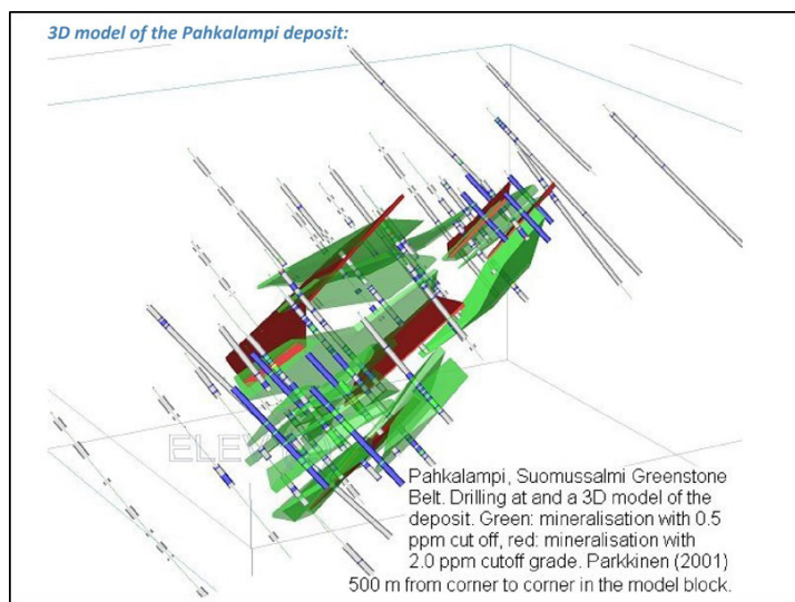
Figure 23: 3D model of the Pahkalampi Prospect as defined by Nordic Mines AB.
