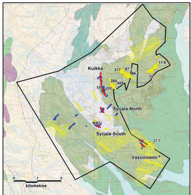
Figure 20: Gold mineralisation at Syrjälä
