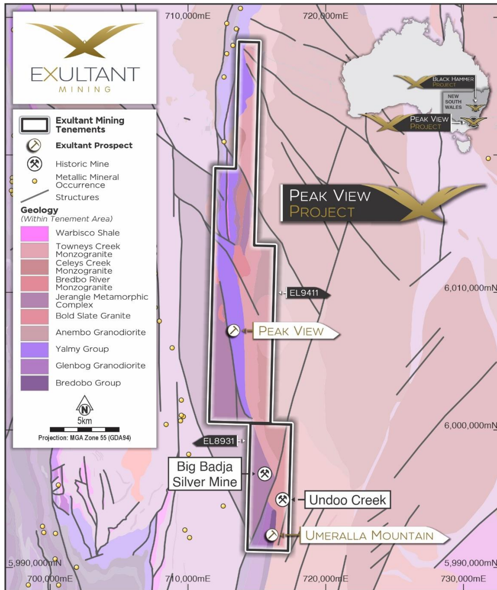
Figure 3. Peak View Project - Regional geology showing key prospect locations
