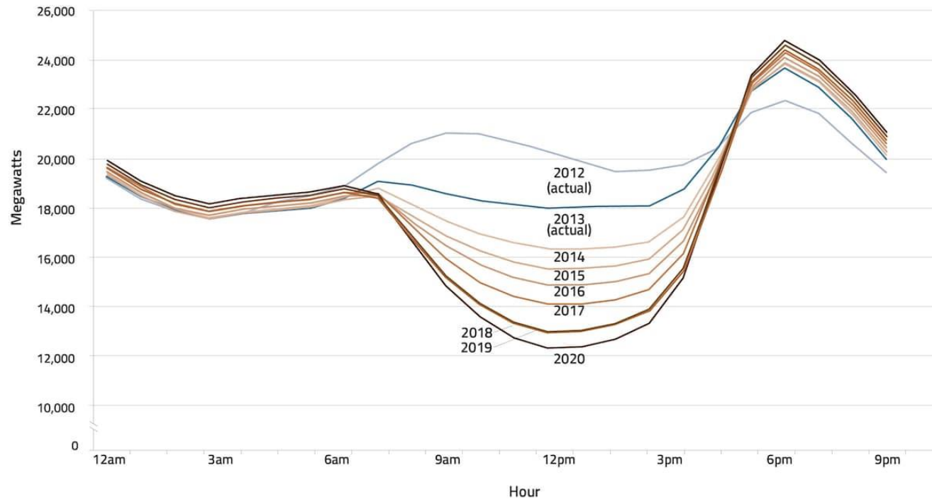
Electricity “Duck Curve”
