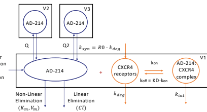
Fig. 4. A 3-compartmental model with parallel linear and non-linear elimination (Michaelis-Menten approximation) as well as explicit receptor binding + complex internalization was able to fit the PK and CXCR4 RO observations more accurately than any simpler model
