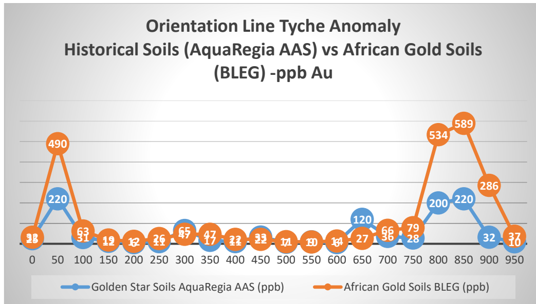
Figure 3: Agboville Project Tyche Prospect – Orientation soil line across center of anomaly showing comparison between historical soils (Aqua Regia AAS) and Recent soils (BLEG) – approximately the same location.
