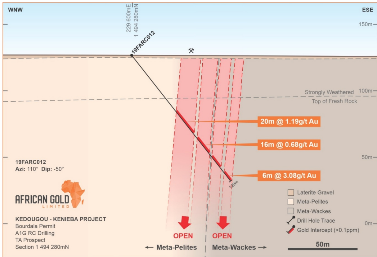
Figure 5: TD Prospect. Schematic Section RC Hole 19FARC012
