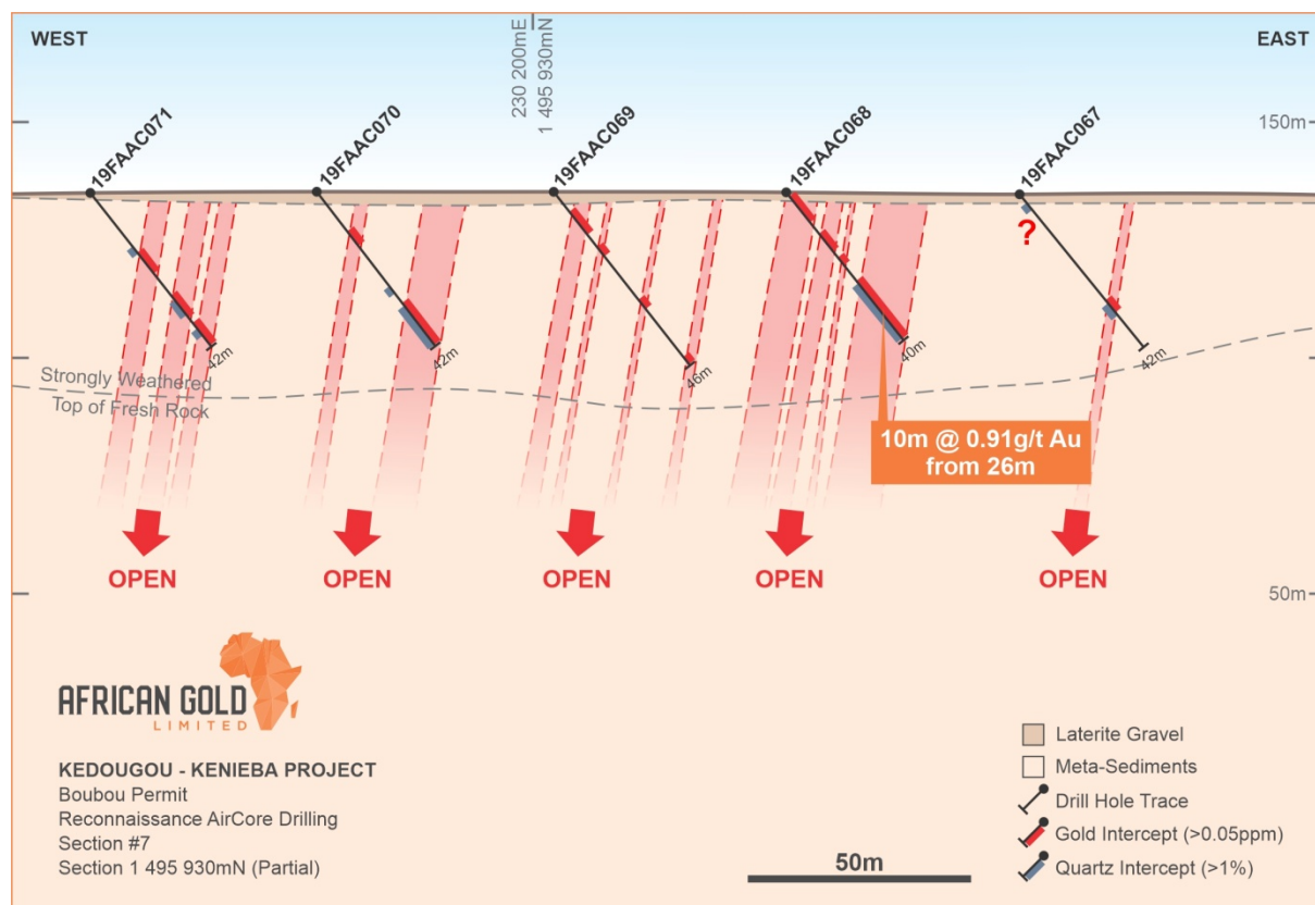
Figure 8: Schematic Section Air Core Drilling for location refer figure 2
