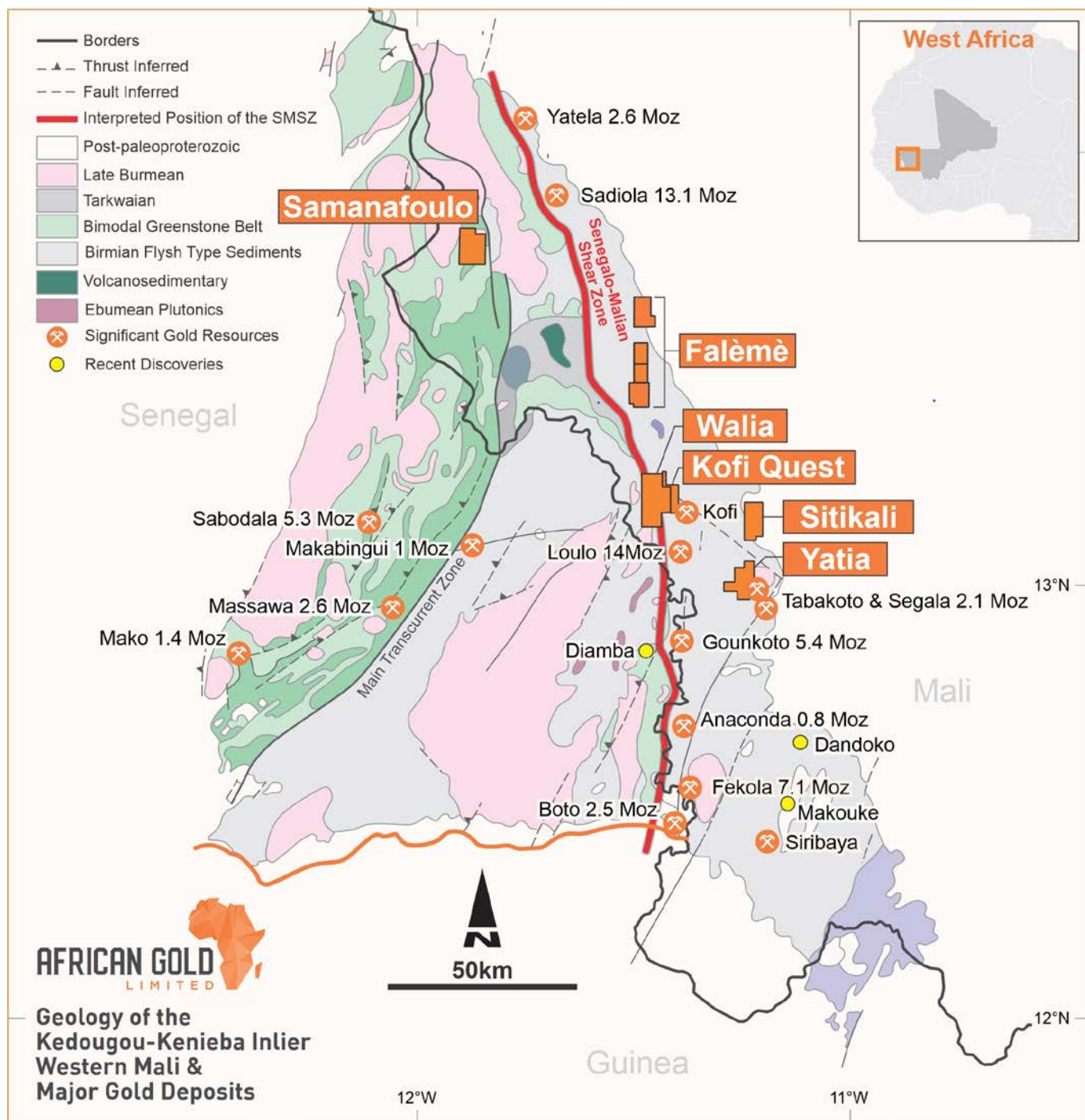
Figure 2: A1G Kedougou Kenieba inlier projects over simplified KKI geology and significant gold deposits.
