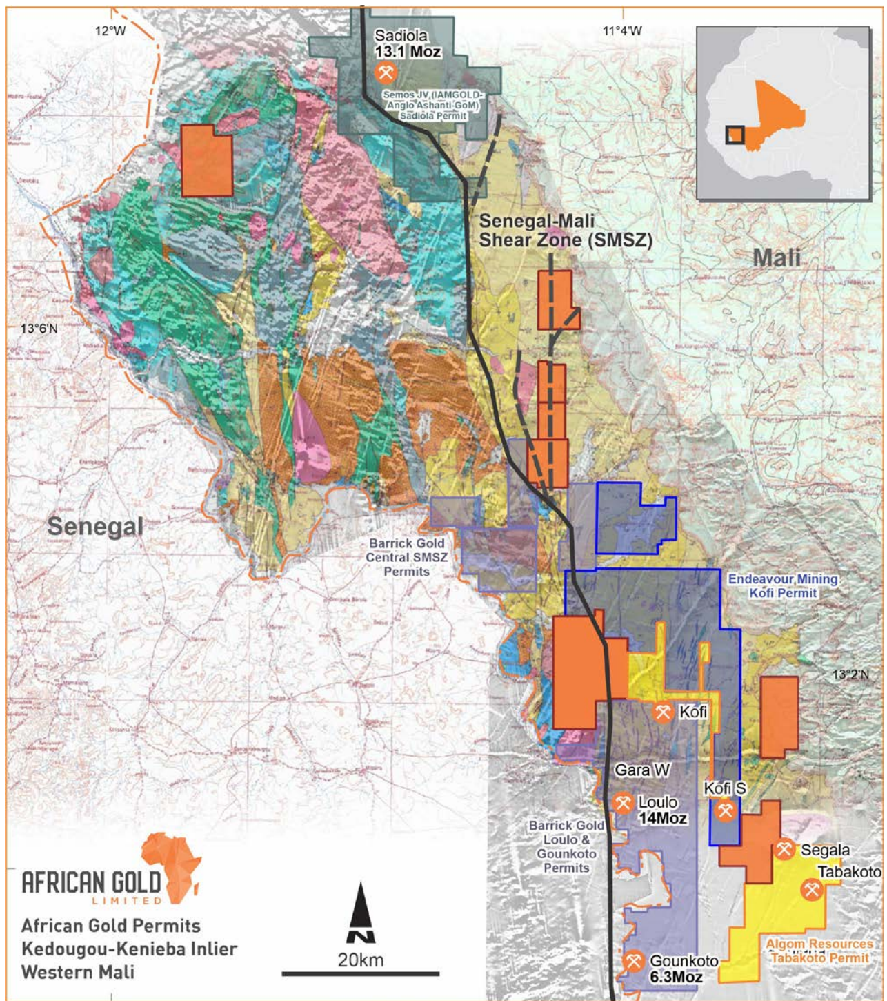
Figure 5: African Gold Limited and Major permits within the norther ½ of the Malian side of the KKI showing geology on magnetics with major producing mines.
