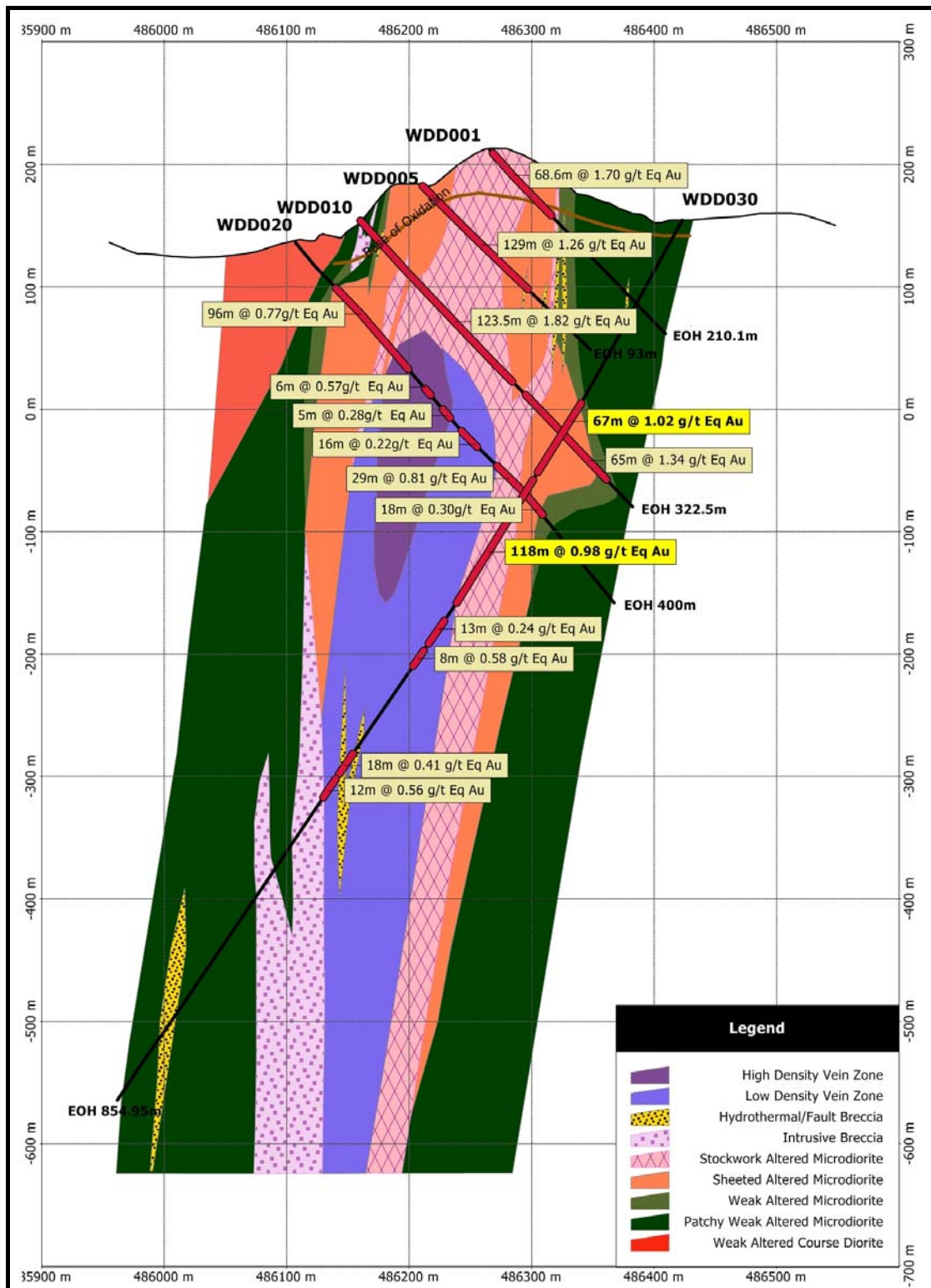
Cross section of diamond drill holes WDD001, WDD005, WDD010, WDD020 and WDD030 showing the extent and zones of gold and copper mineralisation. Mineralisation remains open at depth. Mineralisation widths are drilled widths. Gold is reported as gold equivalents.
