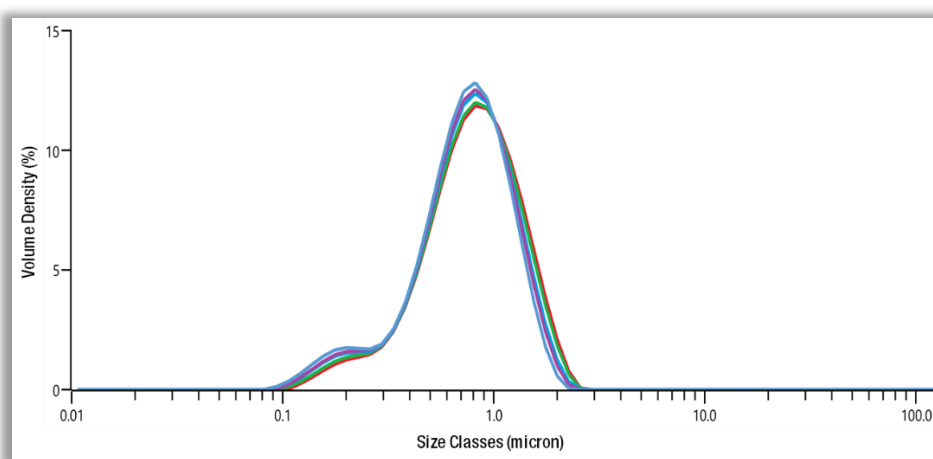
'Battery grade' particle sizing distribution for alpha form HPA powder, achieved without jet milling
