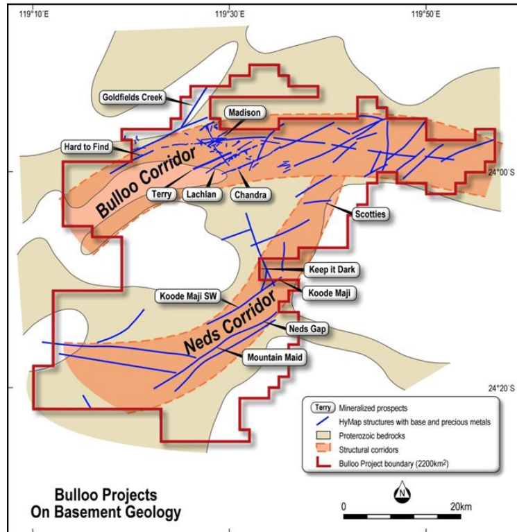
Figure 2 Bulloo Copper Project leases on geology with structures
