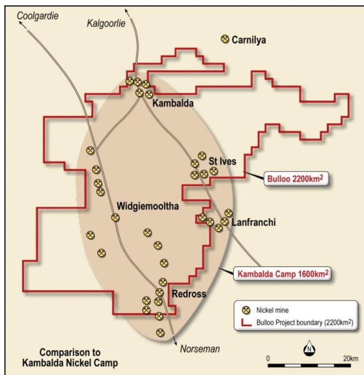
Figure 3 Bulloo Copper Project compared to Kambalda Nickel camp
