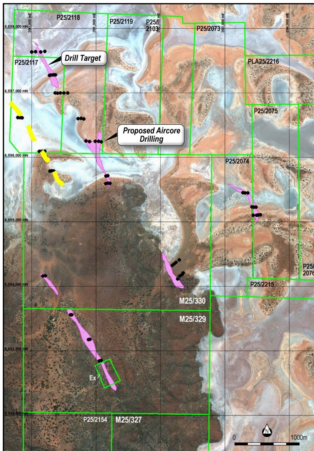
Figure 4 Google ® image with Fluid Flow drilling targets at Glandore
