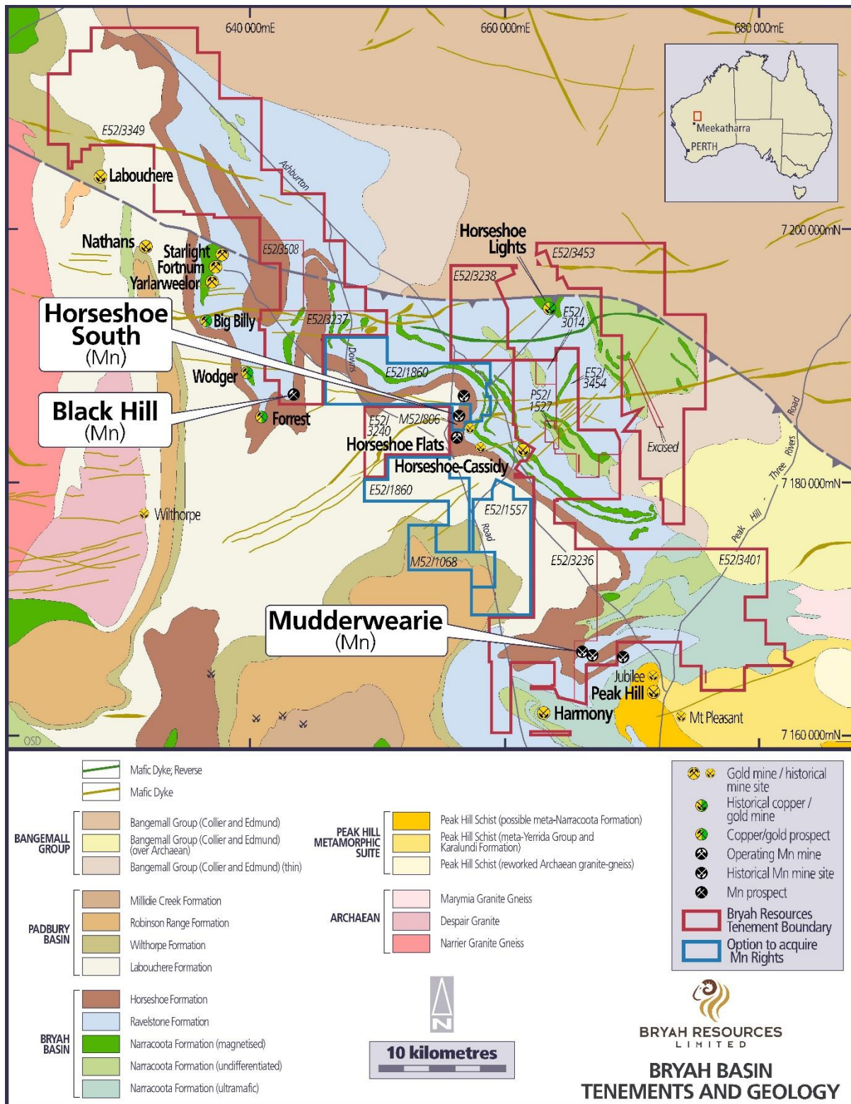
Figure 1 – Bryah Basin Tenements and Regional Geology Map
