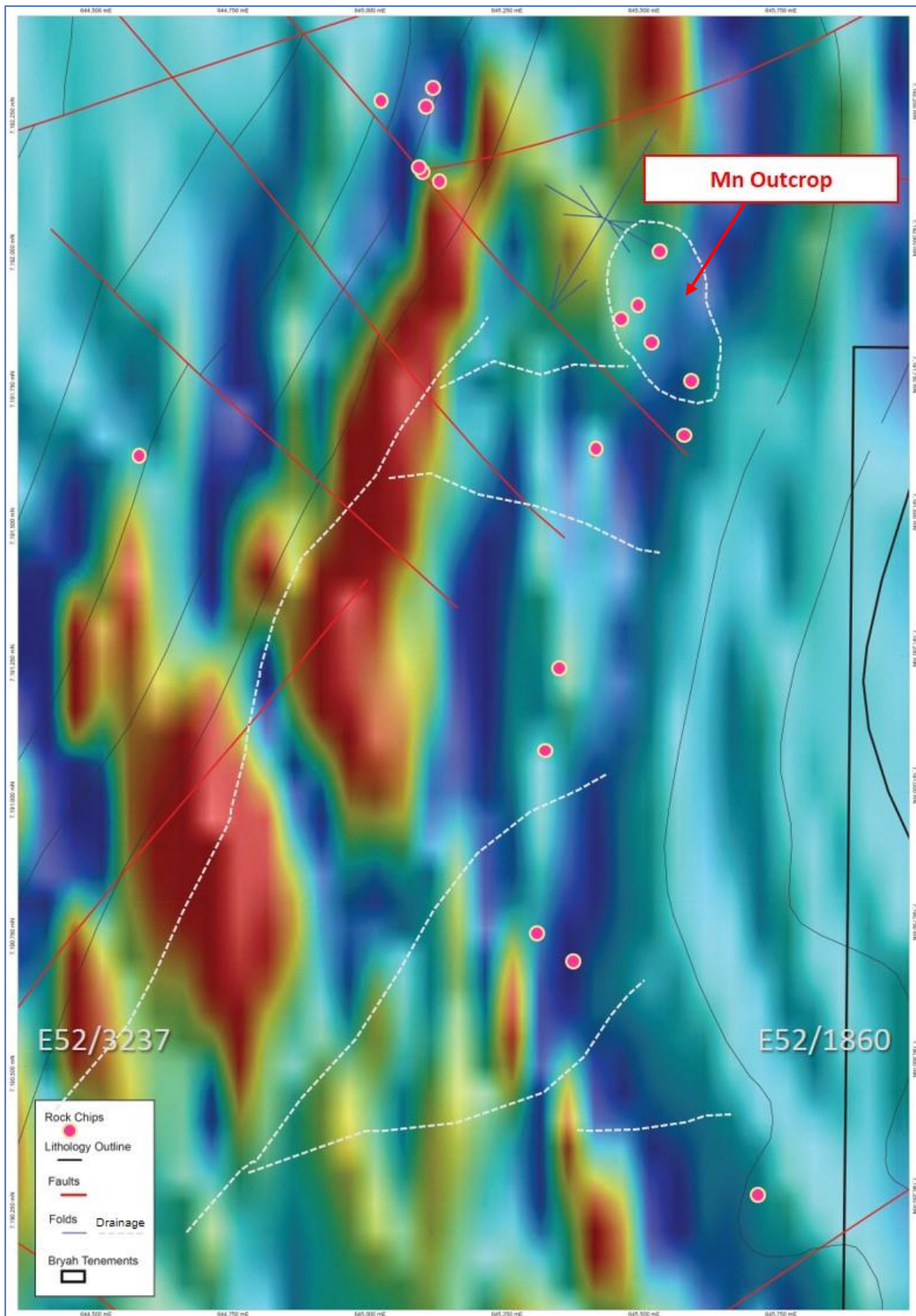
Figure 5 – VTEM Imagery (VTEM18_BFz_Ch28_1vd_psc_ne) showing Brumby Creek Prospect
