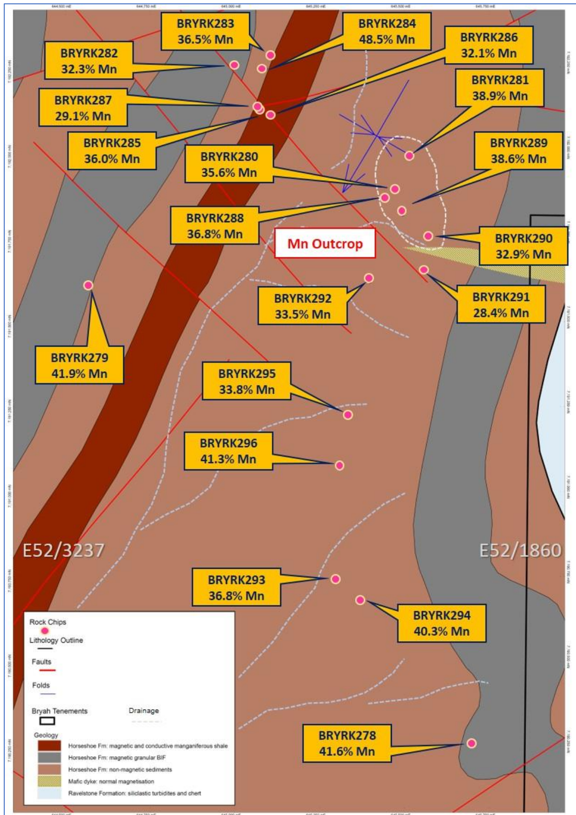
Figure 4 – Brumby Creek Prospect Interpreted Geology showing sample locations and results.
