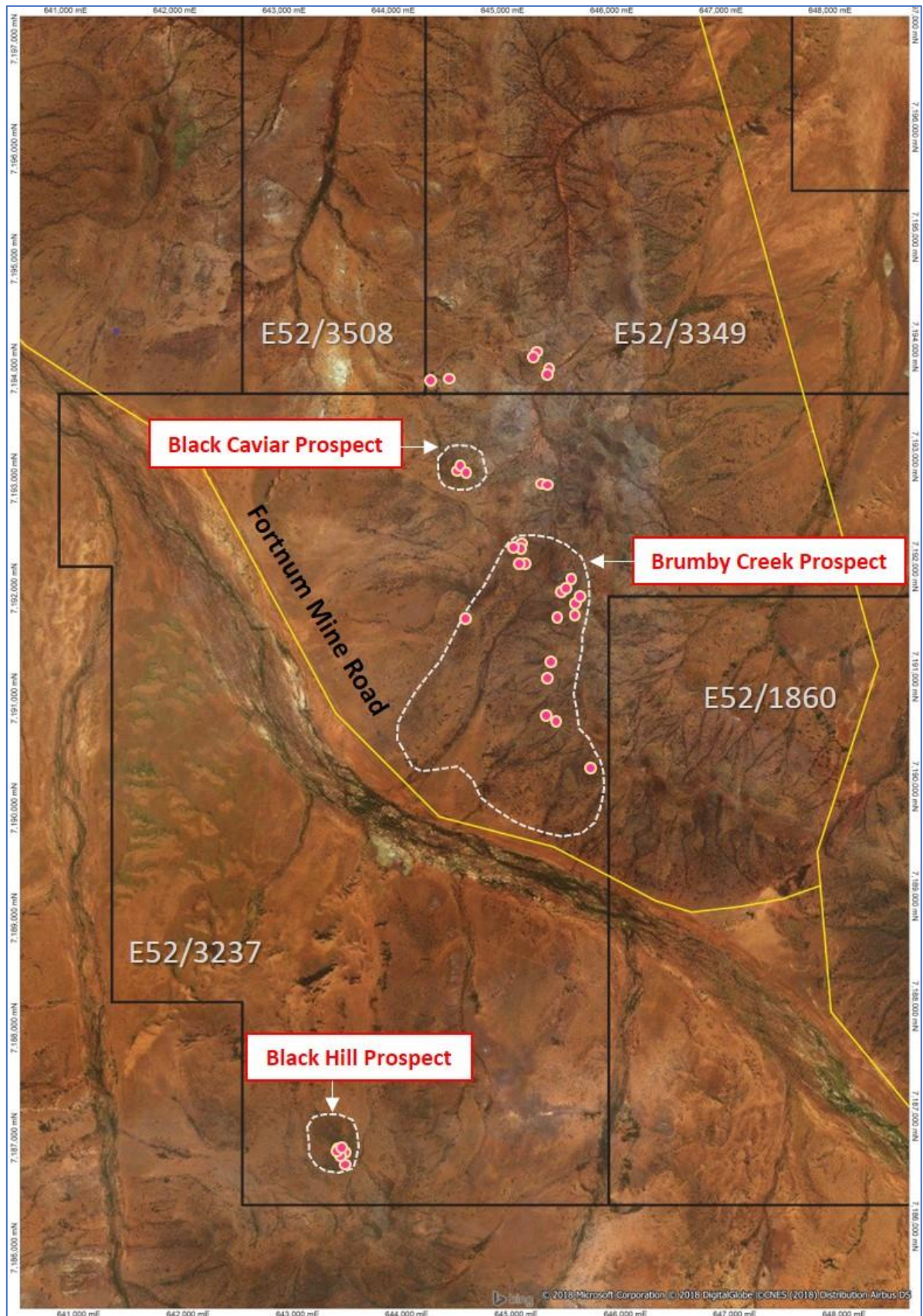
Figure 2 – Satellite imagery showing Brumby Creek and other nearby Prospects and rock chip sample points
