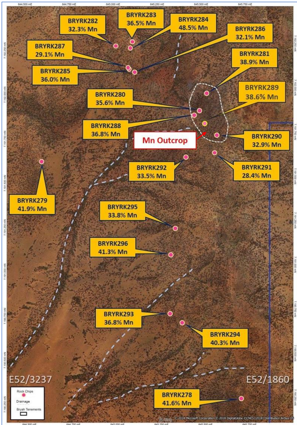
Figure 3 – Satellite imagery showing Brumby Creek Prospect, sample locations and results.
