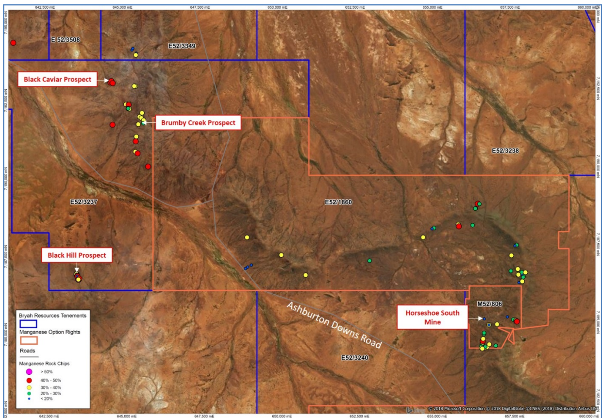
Figure 3 – Northern Bryah Basin Tenements and Manganese samples
