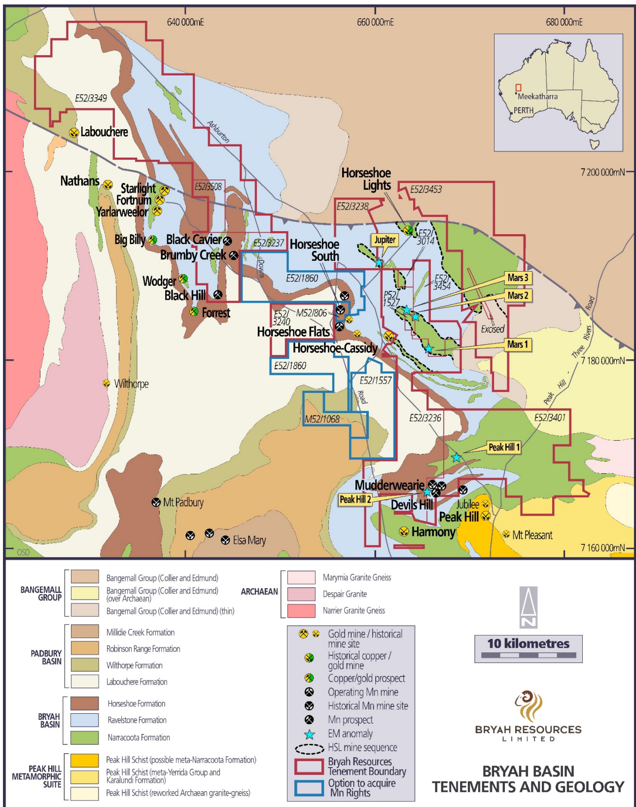
Figure 2 – Bryah Basin Tenements and Geology Map showing EM anomalies
