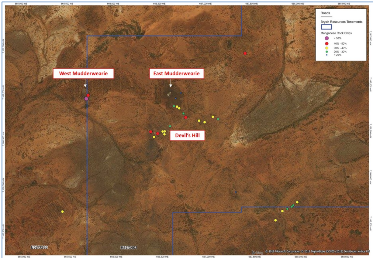
Figure 4 – Southern Bryah Basin Tenements and Manganese samples
