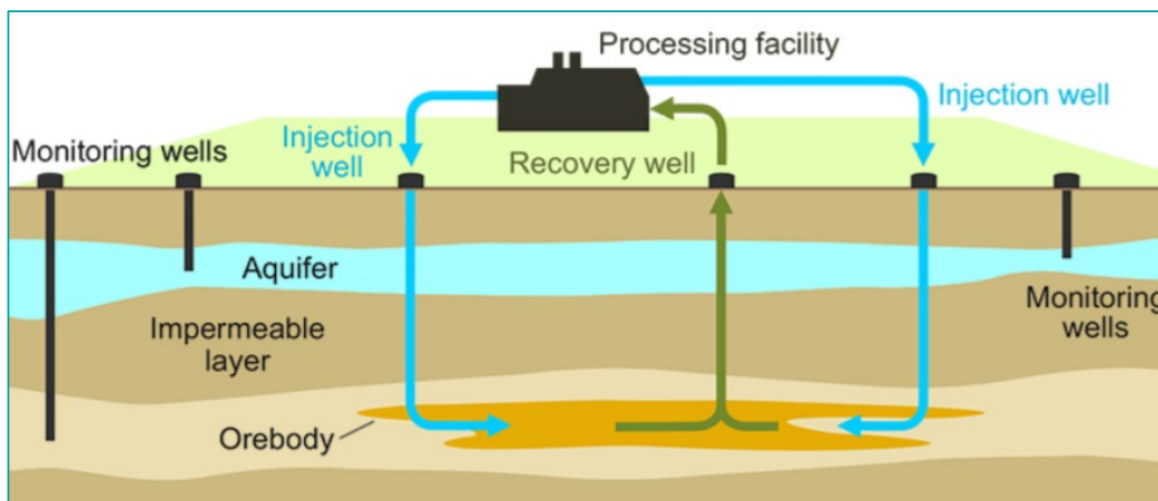
Figure 4: In-situ leaching
