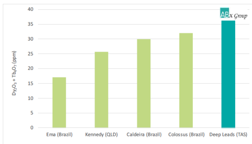
Figure 2: Deep Leads REE Project Dy+Tb grades compared to global ionic adsorption clay projects (data shown in Table 6)
