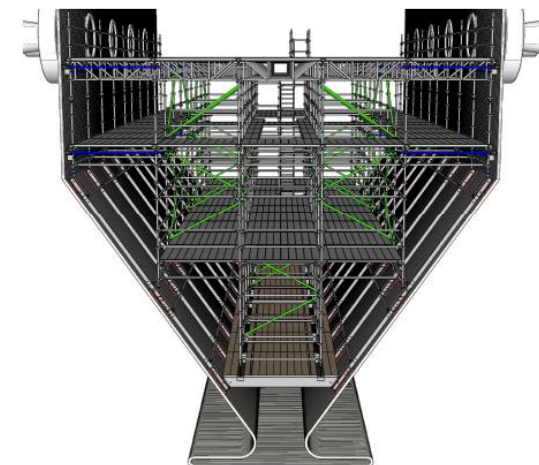
Furnace Kit Schematic
