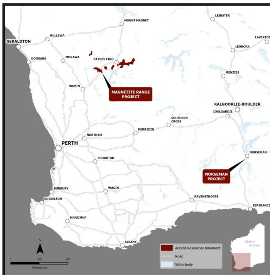
Figure 1 – Accent Resources Project Location Map Magnetite Range Project (ACS 100%)
