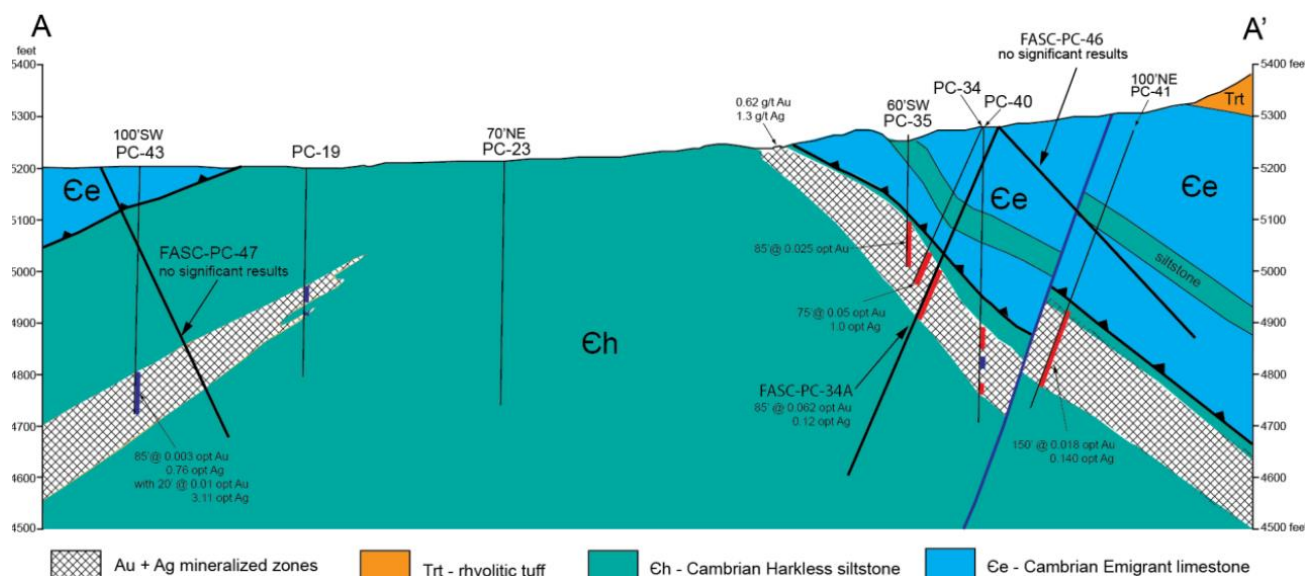
Figure 6 - Section view A-A' (refer to figure 4)
