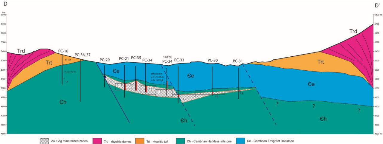
Figure 5 - Section view D-D' (refer to figure 4)
