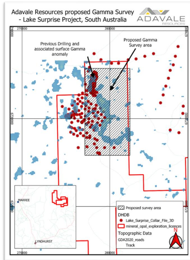
Figure 1: Area of gamma survey and rock chip sampling
