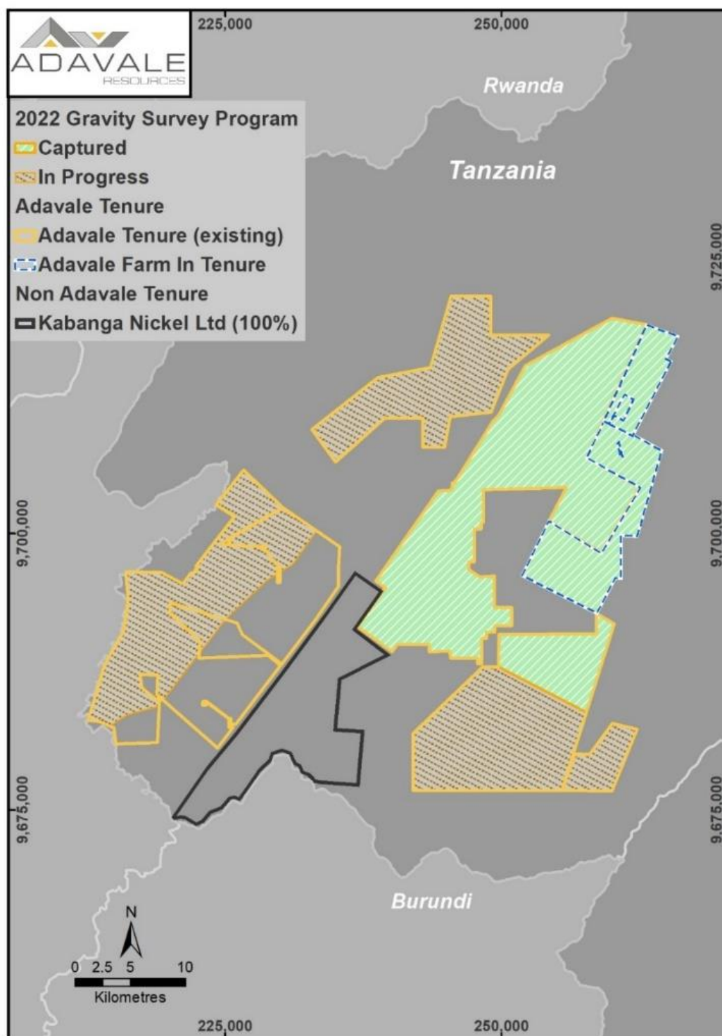
Figure 2: Summary of gravity surveys completed and remaining areas in progress
