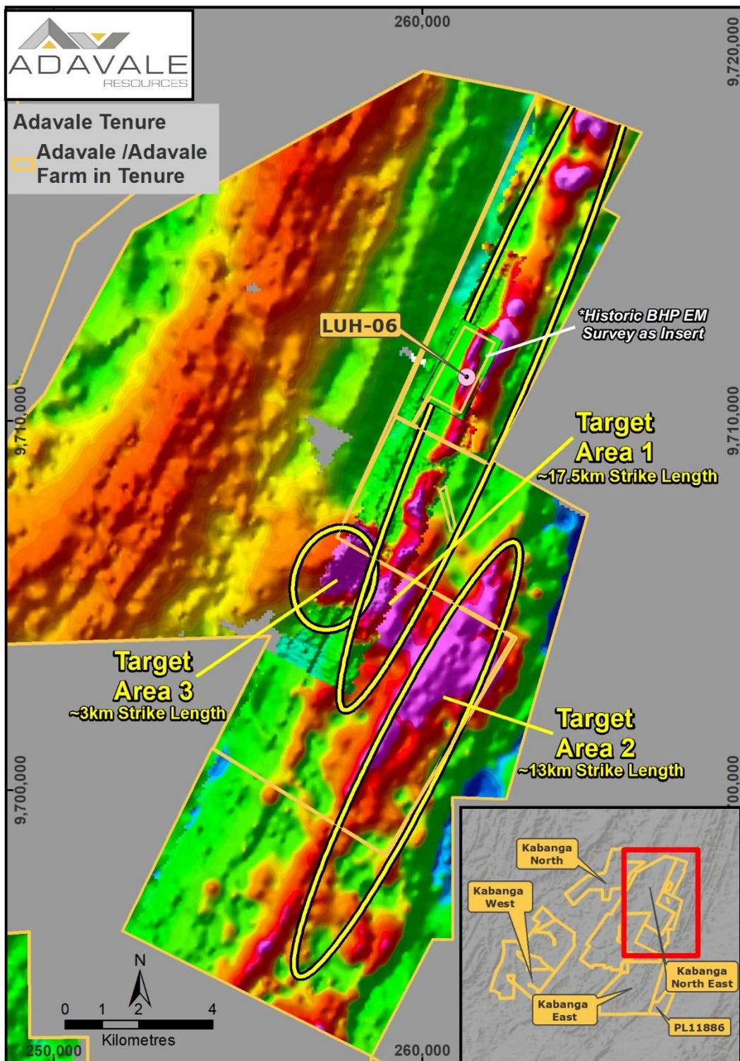
Figure 1a: Target areas within Luhuma Corridor and the newly discovered Target Area 2 (Note that the Luhuma corridor on the right has been enhanced separately from the Kabanga NE area on the left in order to better define localised gravity targets)
