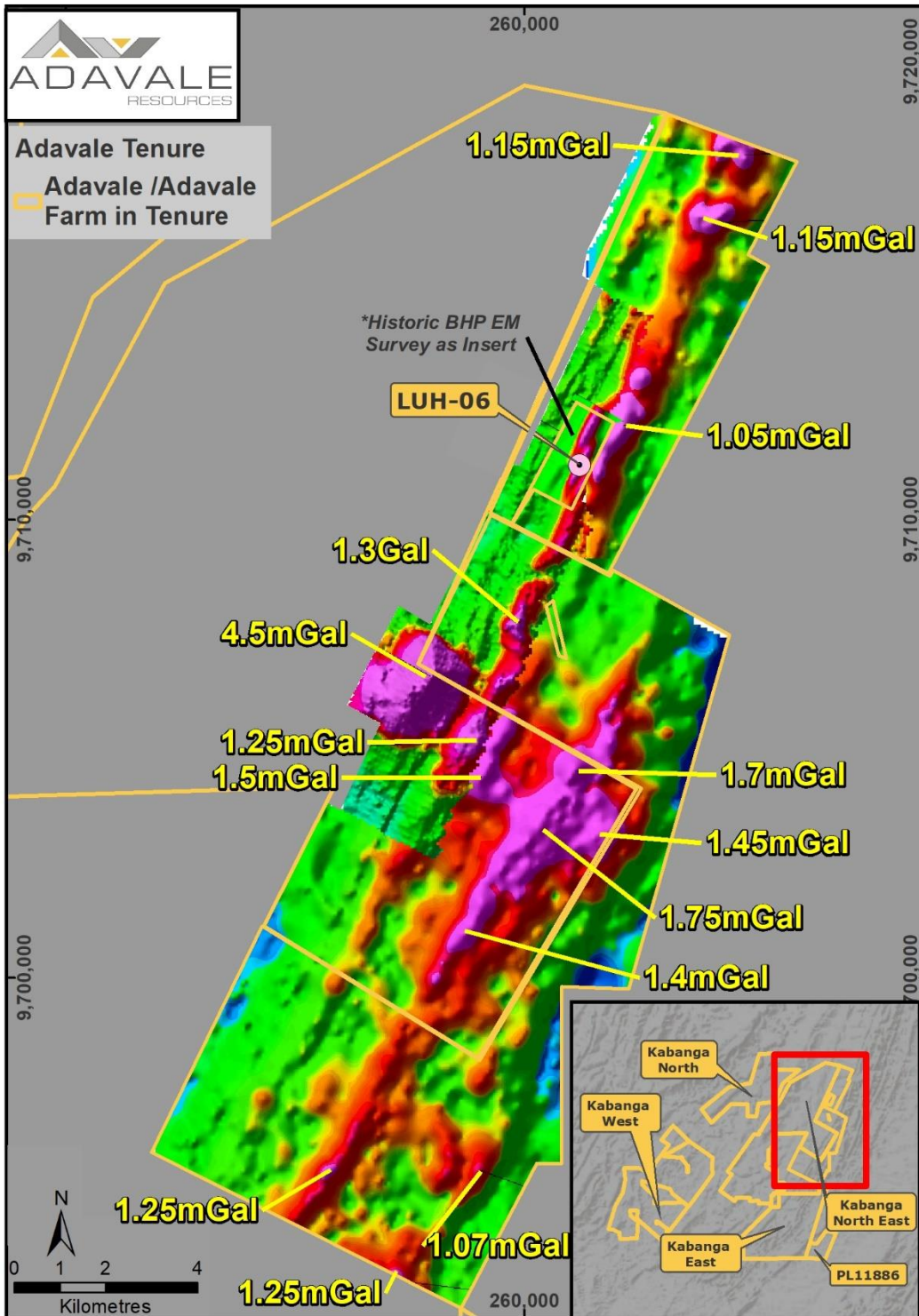
Figure 1b: Location of the 14 discrete high density high priority targets within the Luhuma Corridor
