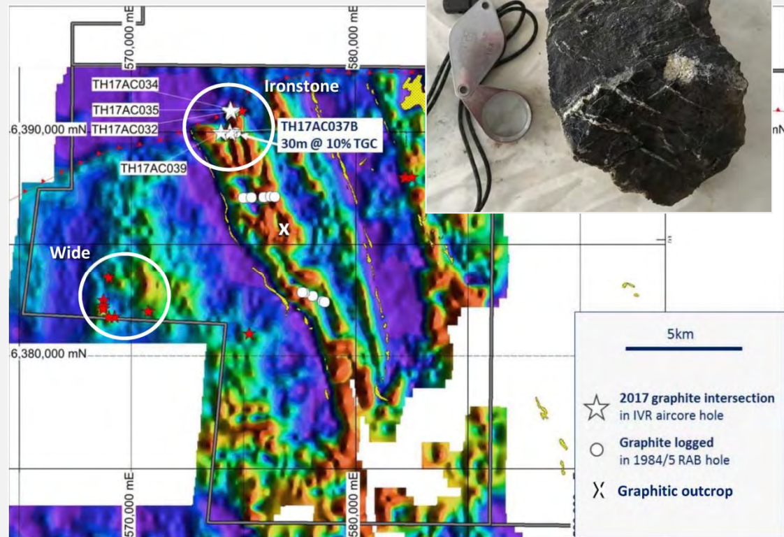
RepTEM conductivity image showing graphite occurrences
