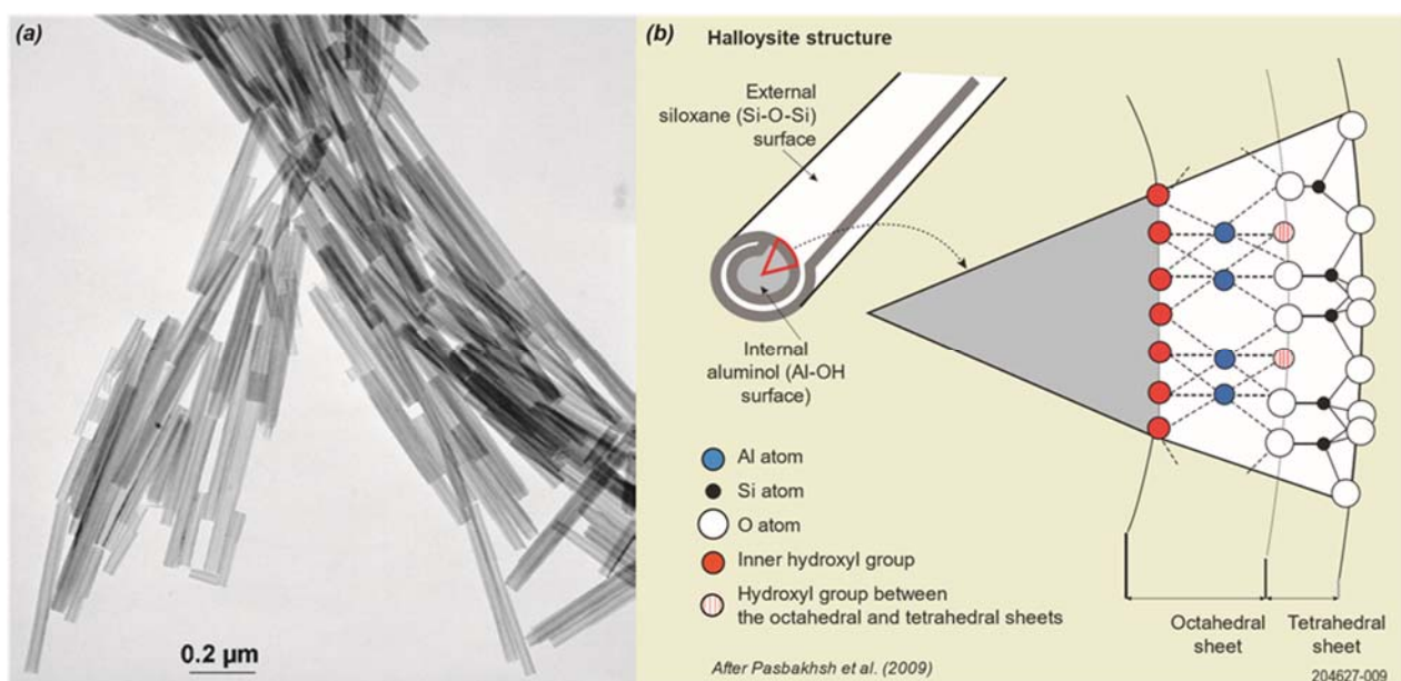
Figure 4 - (a) Extremely Regular Halloysite Nanotubes from Camel Lake (b) Halloysite Crystal Morphology and Atomic Structure
