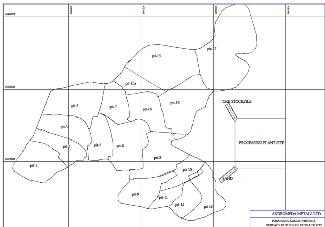
Figure 7 – Mining Stages
