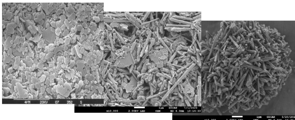
SEM photographs illustrating varying halloysite:kaolinite content of nanoclay samples from the Great White kaolin-halloysite deposit, western South Australia.
