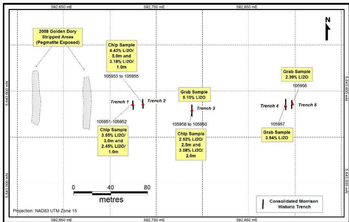
Figure 11. Root Lake Pegmatite due diligence trench sampling by Golden Dory in 2009
