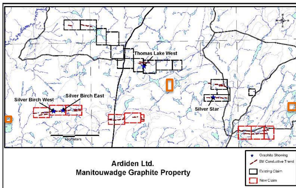
Figure 17: Manitouwadge graphite project showing approx. 20km of EM anomaly strike length and newly staked claim (in orange) along strike from Silver Star North
