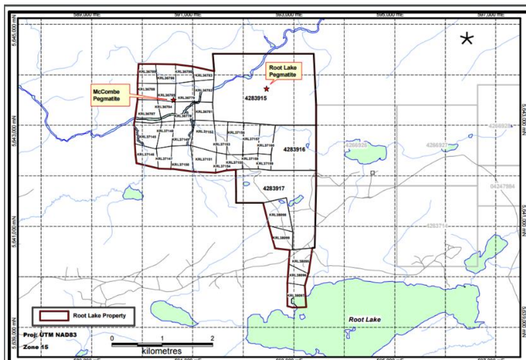
Figure 6: Root Lake Lithium Project Claims Area and location of McCombe Pegmatite and Root Lake Pegmatite
