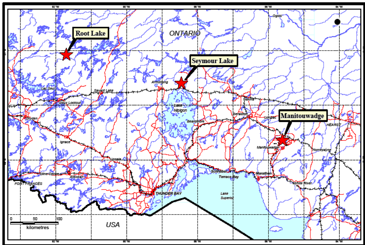
Figure 1: Location of Seymour Lake Project (230km north-northeast of Thunder Bay)
