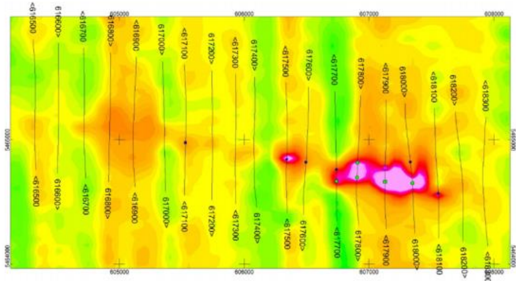
Figure 12: Silver Star North: Target EM12 image of 900Hz VCA in-phase response with OGS anomaly picks
