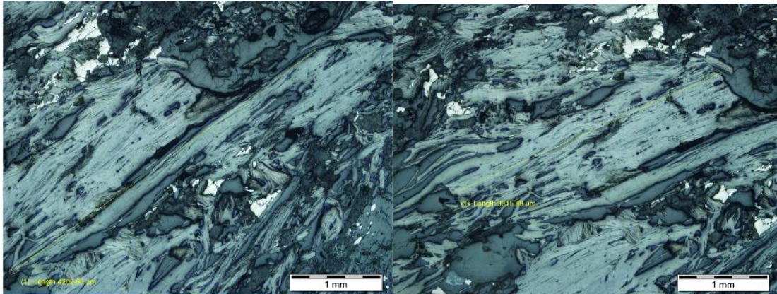
Figure 15: Petrographic slices from EM 12-05 – Flake size of 4,209 micron on left and 3,315 micron on right. Super jumbo graphite is defined as graphite with a flake size of >500 microns. (Source: Vancouver Petrographics)
