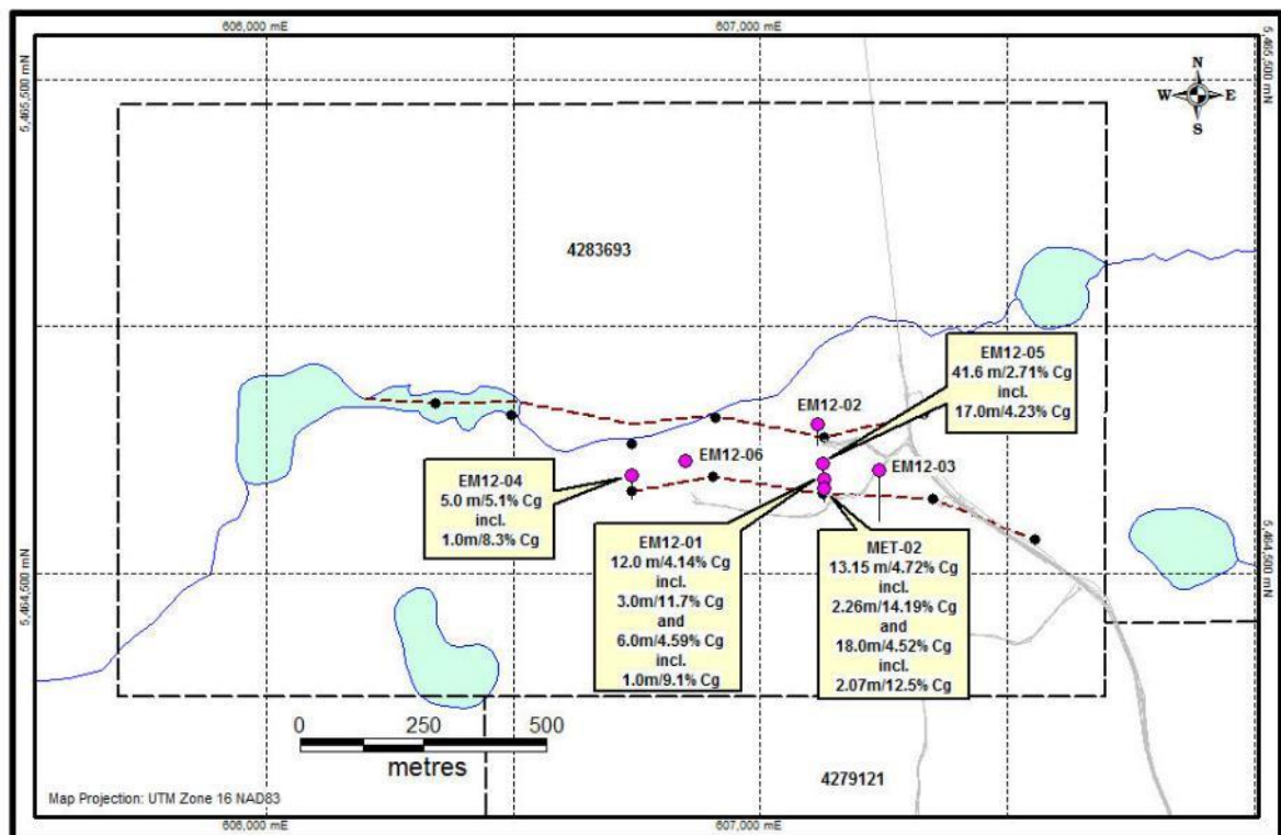
Figure 13: Silver Star North with drill holes and grades noted
