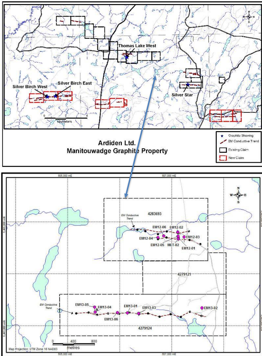
Figure 14: Manitouwadge Graphite Project showing 19km of EM anomalies (in red in upper diagram)) with graphite prospectivity. Silver Star North (EM12) prospect is shown as one of the Eastern EM anomalies
