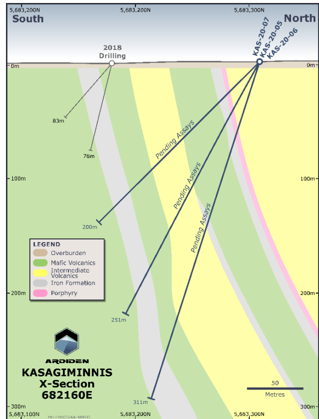
Figure 6 – Cross Section of Drilling from Pad 3- pending results
