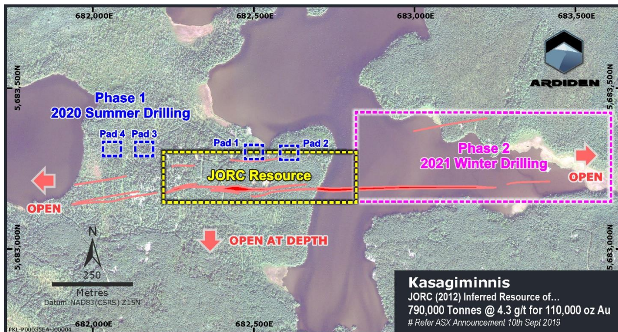
Figure 1 - Drill pads completed at the Kasagiminnis Gold Deposit
