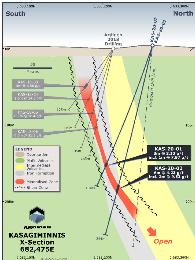
Figure 5 – Cross Section of Drilling from Pad 1
