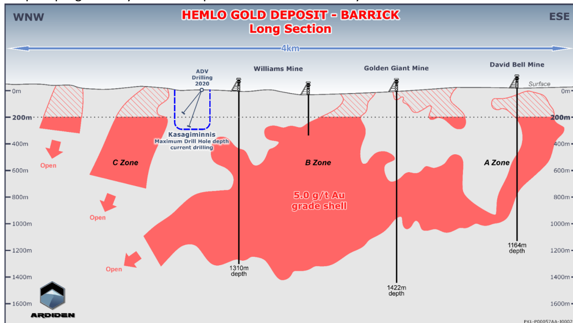
Figure 3 – Long section Hemlo Deposit, Barrick Gold, Ontario
