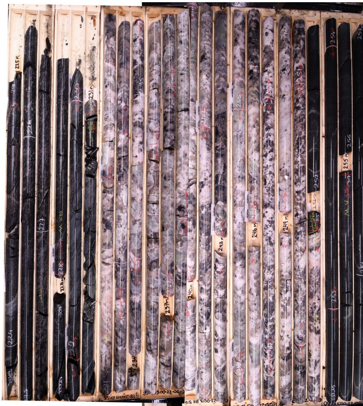
Figure 4: Diamond drill core from hole GTDD-22-0003; thick, high-grade LCT spodumene bearing pegmatite intercept of 19.2m at 2.20% Li 2 O from 231.8m
