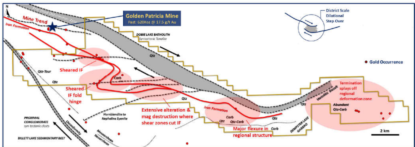
Figure 8 -- New Patricia - Structural Interpretation Plan
