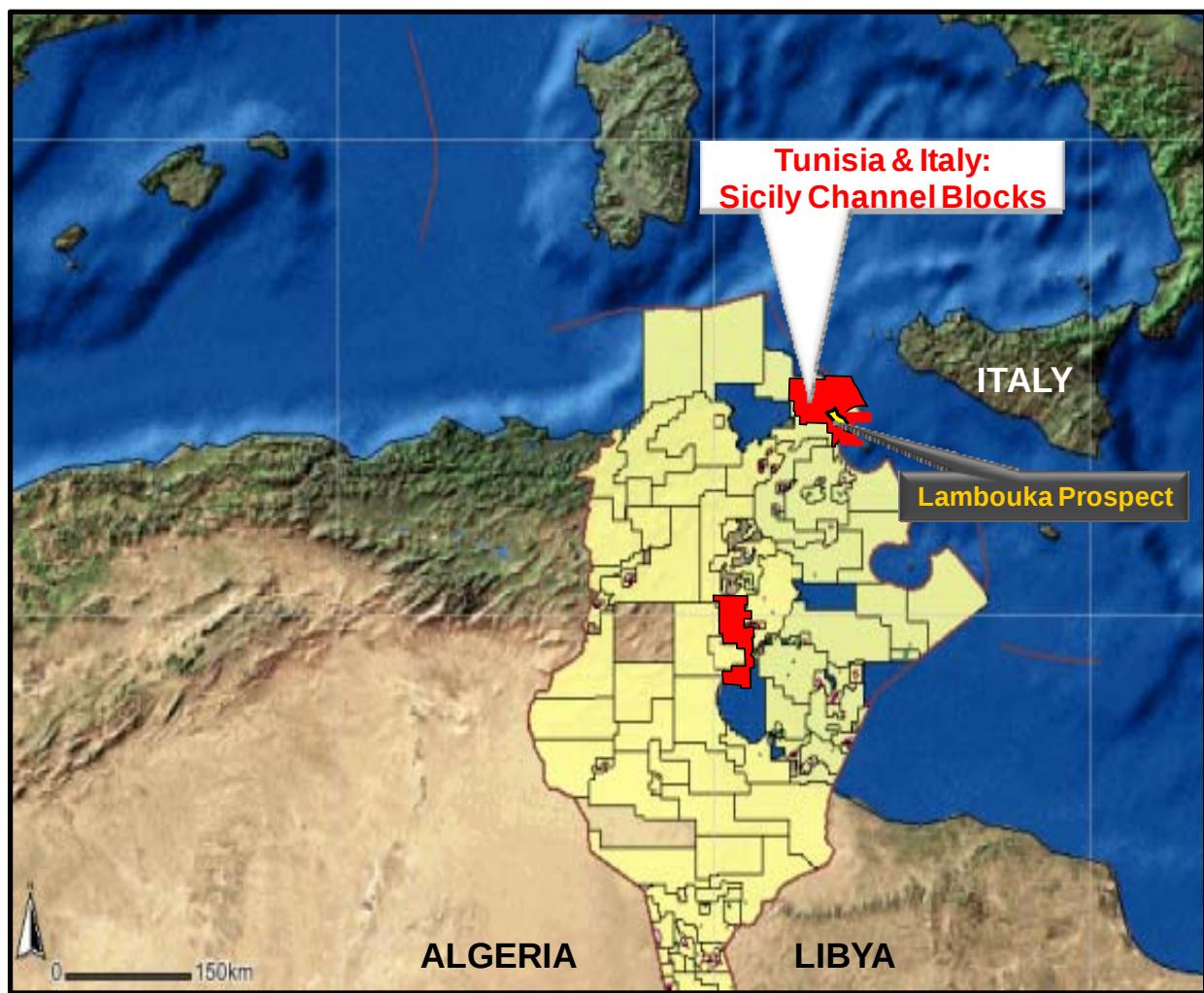
Map showing AuDAX licenses in Tunisia and Italy in red.
