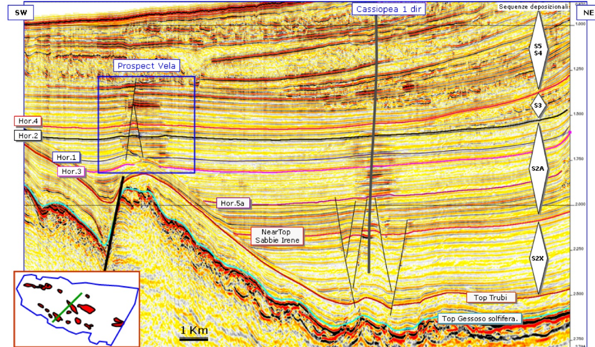
NEW 3D SHOWING CASSIOPEA FIELD AND VELA PROSPECT
