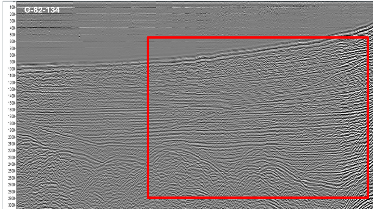
LEGACY 2D LINE 80s ACROSS CASSIOPEA FIELD
