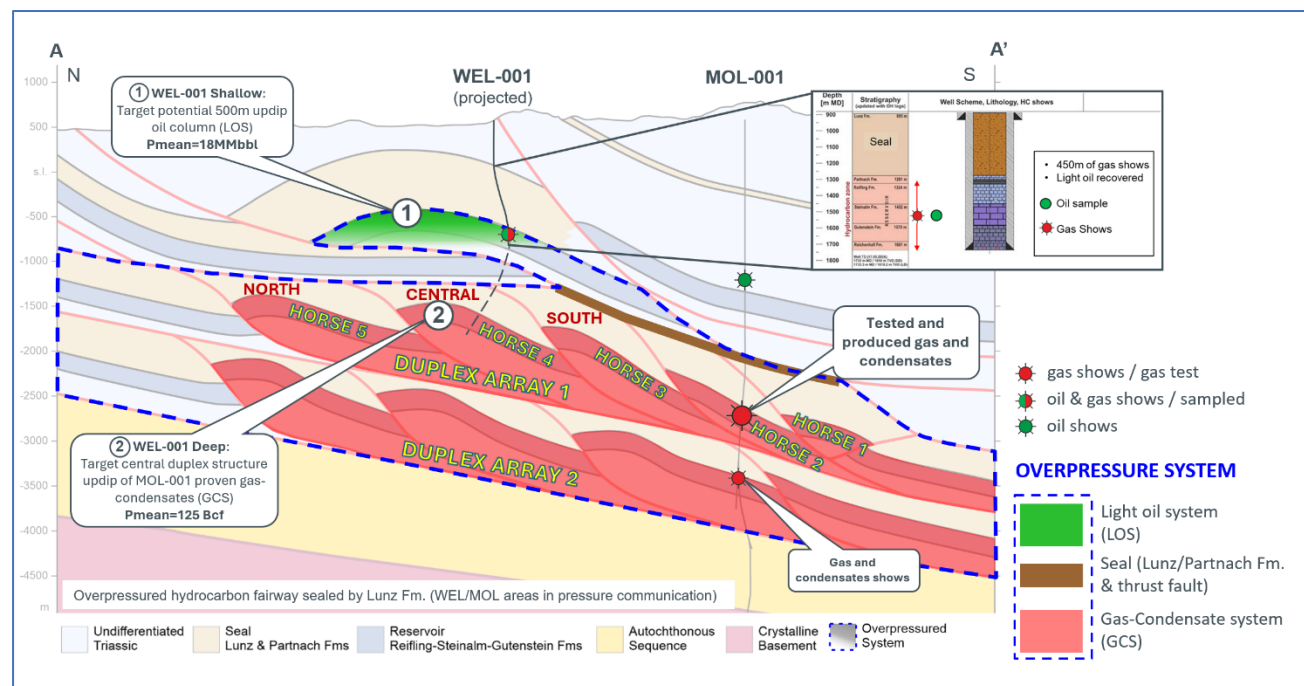
Figure 2: Shows the interpreted oil water contact for the updip light oil accumulation located in the Reifling Formation at the WEL-001 well (1) and the deeper duplex structure updip of the Moln 1 discovery well (2)
