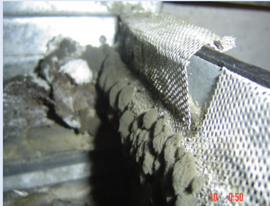
Air-duct supplying room in 5* hotel in Asia
