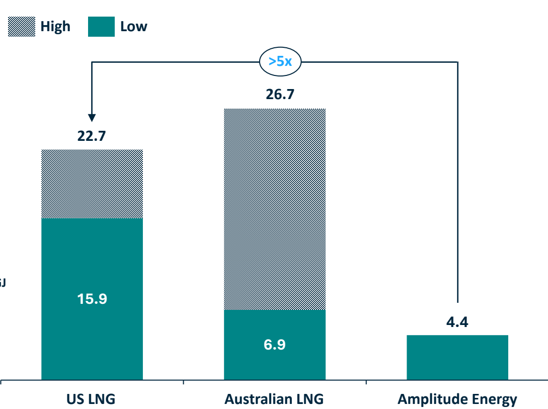
Emissions intensity of producing LNG vs. domestic gas, kgCO 2 -e/GJ 4
