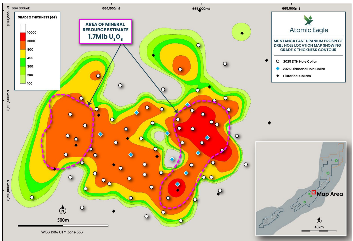
Figure 3: Muntanga MRE outline within Grade x Thickness contour
