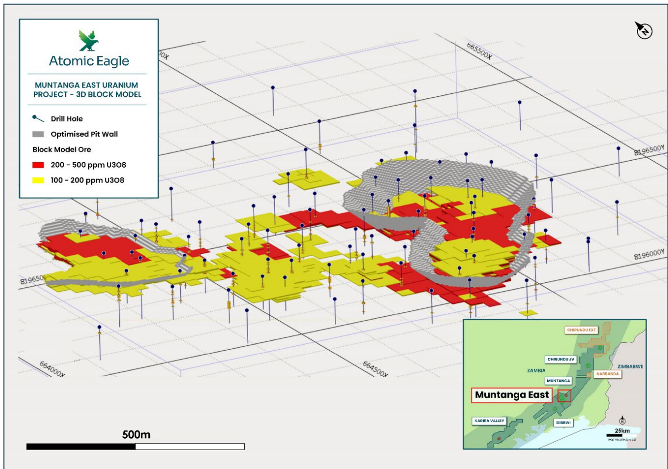
Figure 5: Muntanga East block model 3D view looking northeast of the uranium resources and open pit shells (grey)
