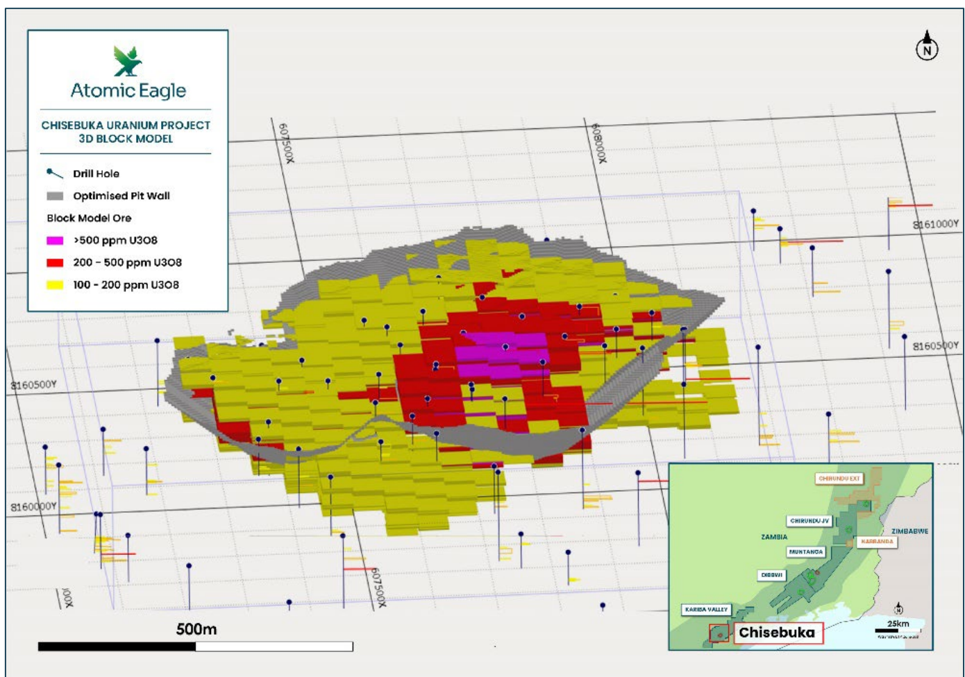
Figure 4: Chisebuka block model 3D view looking northeast of the uranium resources and open pit shells (grey)
