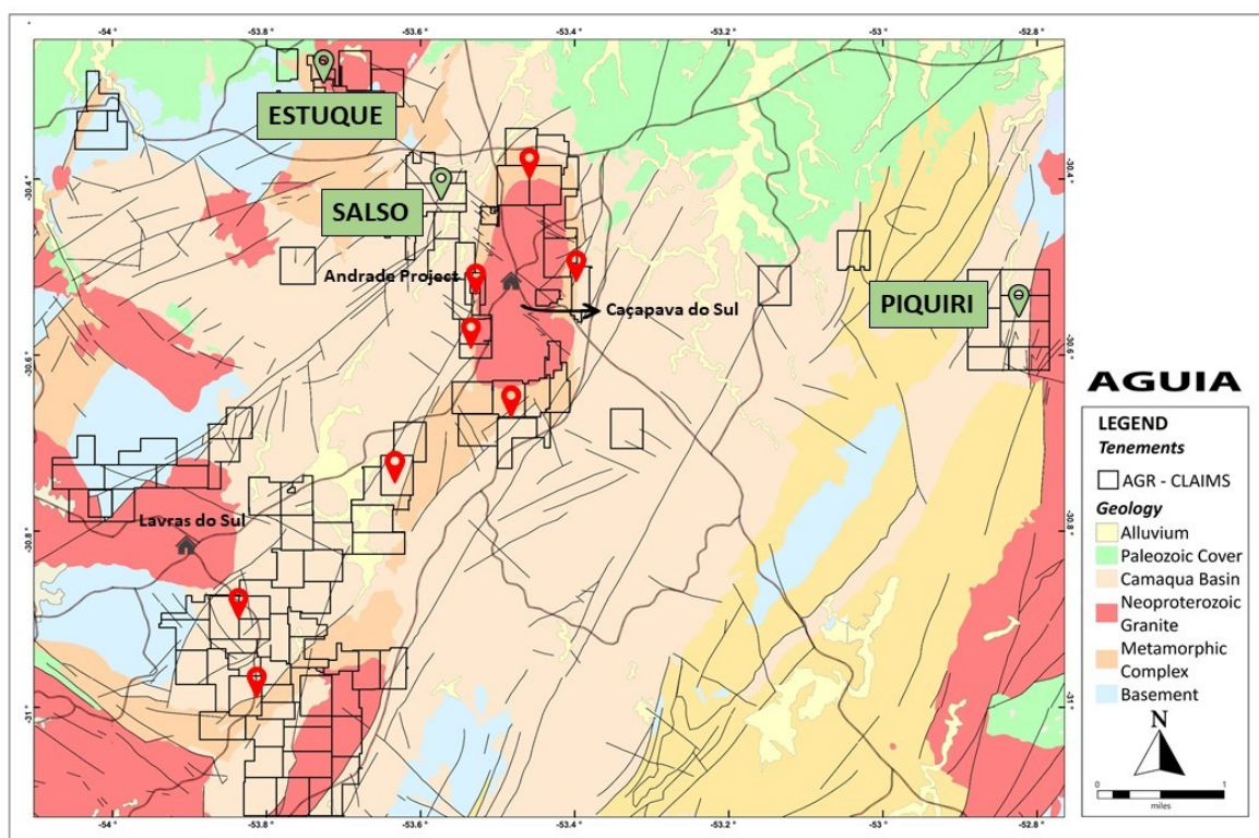
Figure 04 – Regional Geological map of the Rio Grande Copper Belt highlighting the distribution of Agüia's tenements, copper targets, and identified targets: Salso, Piquiri and Estuque.
