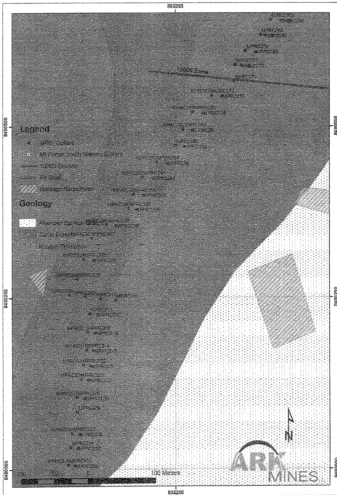
Figure 5: Mt Porter South plan view in MGA 94 grid showing major geological units and drill collar locations.
