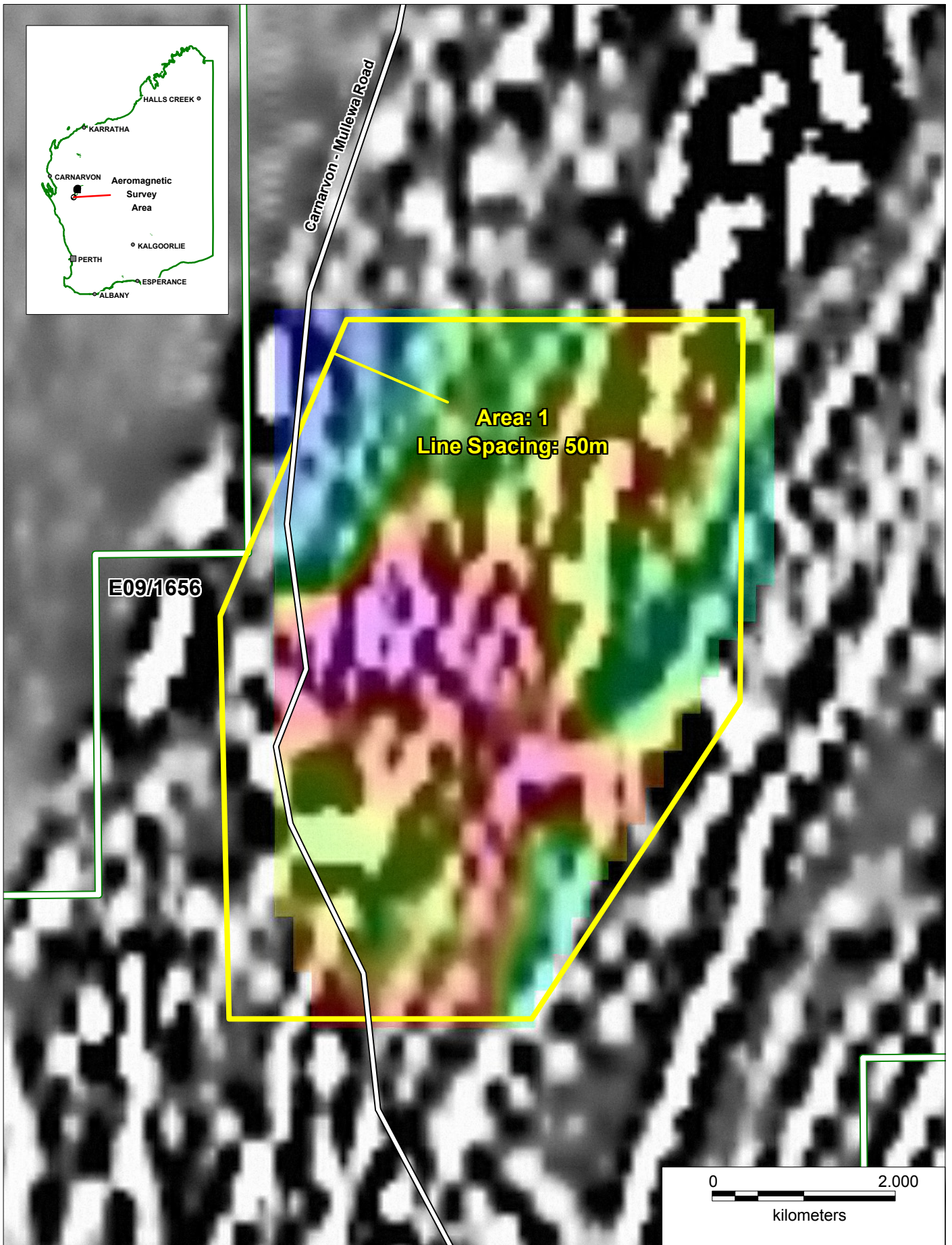
Athena Acquired Residual Bouguer Gravity Overlying Filtered GSWA 400m Line Spacing Aeromagnetic Data
