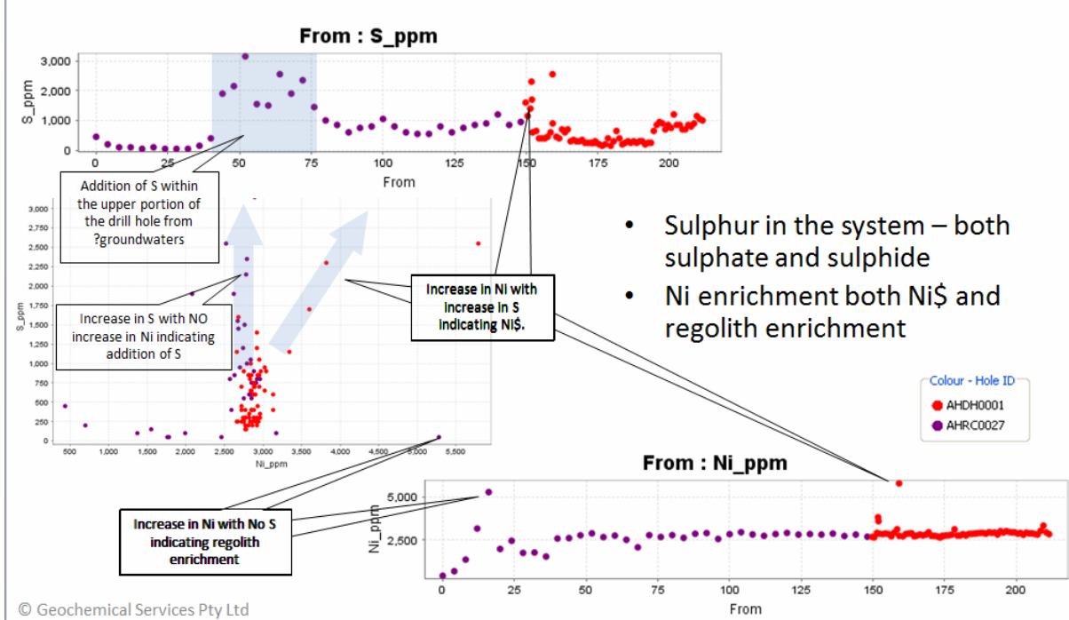
Byro East Intrusion Holes: AHRC0027 and AHDH0001
