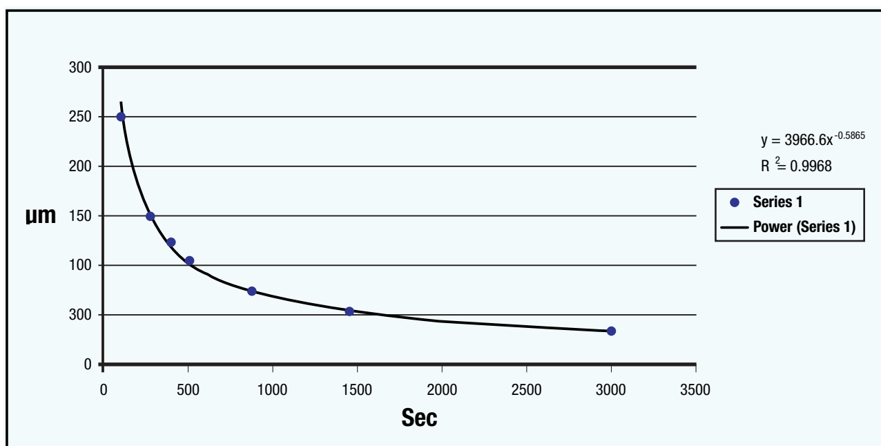
Figure 4. Grind Size Vs. Time to grind in seconds
